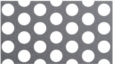
1/4" Diameter 3/8" Staggered Centers / 40% Open Area
